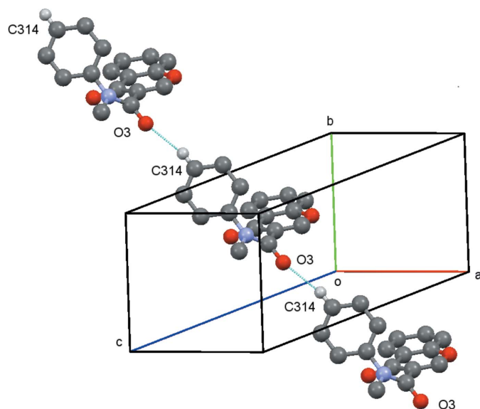
Figure 5 Compound (1): the chain formed by the C314–H314...O3 hydrogen bond. Hydrogen atoms not involved in the hydrogen bonding are omitted.
