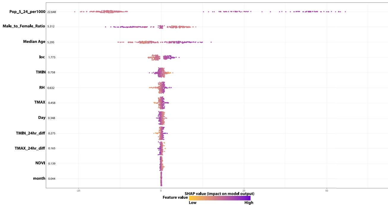
Figure 3. SHapely Additive exPlanations (SHAP) (SHapley Additive exPlanations) values and contributions of the best-performing variables in the best model (generalized additive model). The plot shows the importance of the predictors, with the most important at the top, of the best-performing model using SHAP values. The effect of the contribution is noted as a positive or negative point-level contribution; the given variables' value is represented with a sliding scale from yellow, representing a low variable value to purple, representing a high variable value for each. The x-axis SHAP value illustrates the contribution of every variable to the predicted number of mental and behavioral disorders emergency department visits, with positive values leading to a higher number of predicted emergency room (ER) visits and a negative value leading to a lower number of predicted ER visits.
