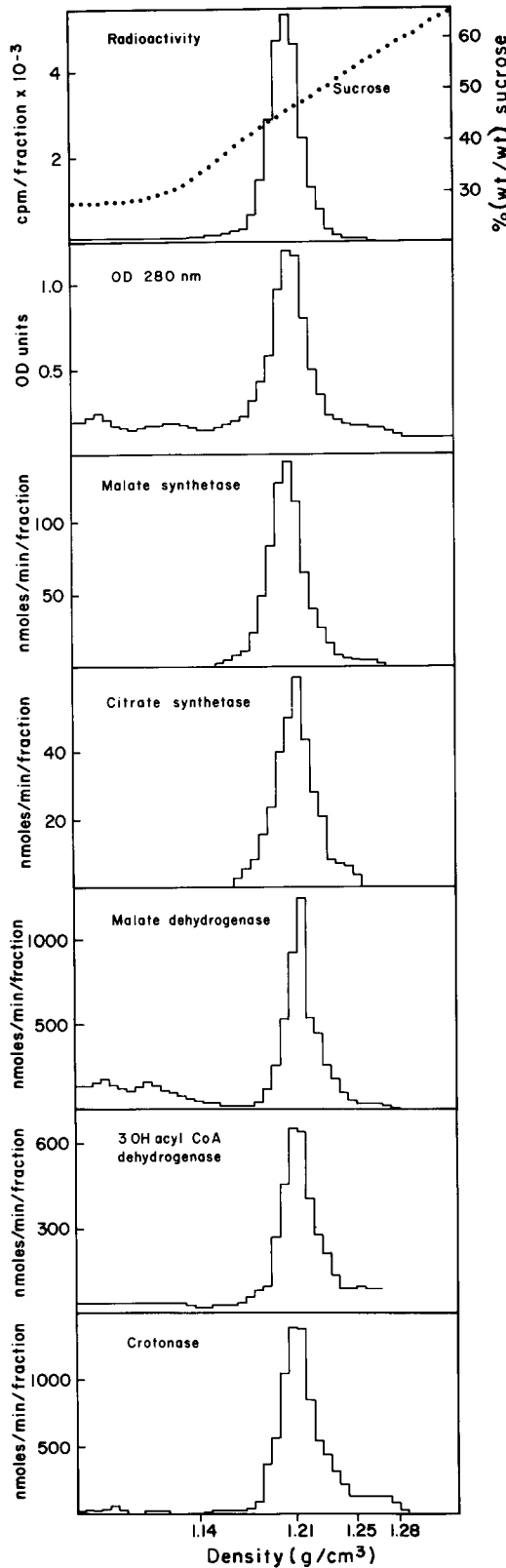
FIGURE 3 Sucrose gradient centrifugation of the glyoxysomal fraction after osmotic shock. The radioactivity represents the membrane in which the lecithin had been labeled by previous treatment of the tissue with [ 14 C]choline.
