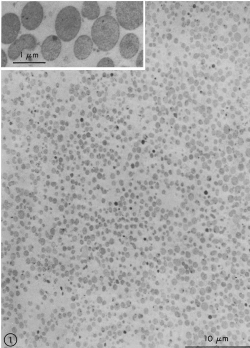
FIGURE 1 Electron micrograph of the glyoxysomal fraction isolated by sucrose gradient centrifugation. The fraction was prepared and fixed as described (16) (courtesy of Dr. T. Moore). Bar represents 10 \mu\text{m} . Section was stained with lead citrate. \times 3,700 . Inset shows several glyoxysomes at higher magnification. \times 18,000 .
