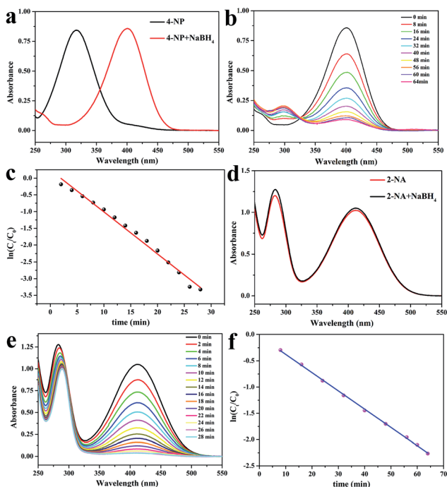
Fig. 7 UV-Vis spectra of 4-NP before and after adding NaBH 4 (a), UV-Vis spectra for the catalytic reduction of 4-NP (b), plots of ln(C t /C 0 ) versus t for the catalytic reduction of 4-NP (c), UV-Vis spectra of 2-NA before and after adding NaBH 4 (d), UV-Vis spectra for the catalytic reduction of 2-NA (e), plots of ln(C t /C 0 ) versus t for the catalytic reduction of 2-NA (f).
