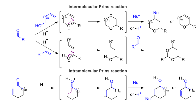
Scheme 1. General Scheme for the Prins Reaction
