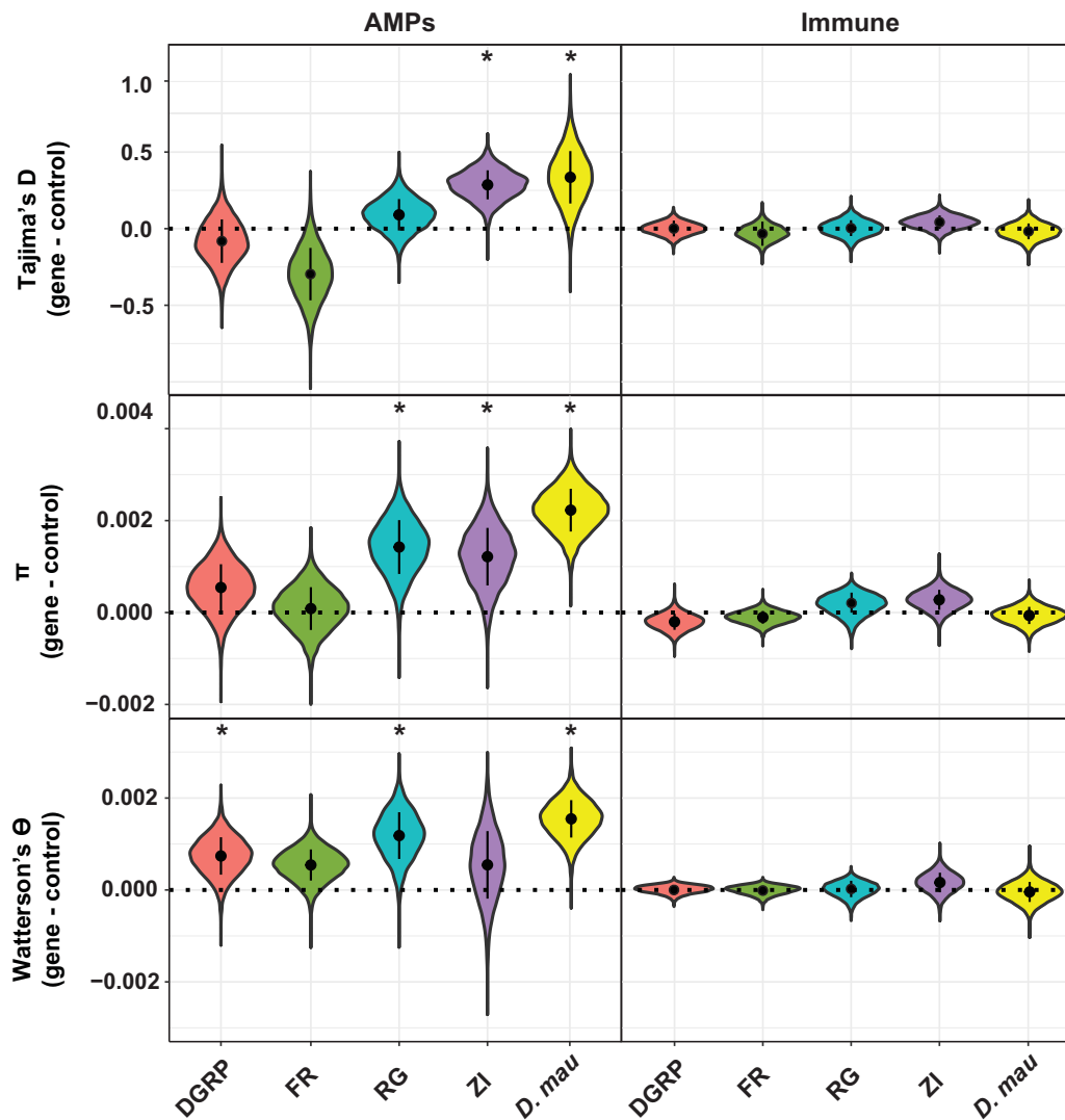
Fig. 1. —Overall, AMPs show more evidence for balancing selection than other immune genes. Difference in means between 35 AMPs and randomly chosen control genes (left-hand side) or 288 immune genes and randomly chosen control genes (right-hand side), resampled 10,000 times, separated by population (DGRP = Drosophila Genetics Reference Panel from North Carolina, USA; FR = France; RG = Rwanda; ZI = Zambia; D. mau , D. mauritiana ). Top panel: Tajima's D ; middle panel: \pi (nucleotide diversity); bottom panel: Watterson's \theta . All three statistics were calculated on silent (four-fold degenerate) sites only. The black dot within each plot shows the median for that population, and the black bar around the dot visualizes the interquartile range of the distribution. Values above 0 are consistent of balancing selection. Asterisks indicate cases where <5% of resamplings have values <0.
