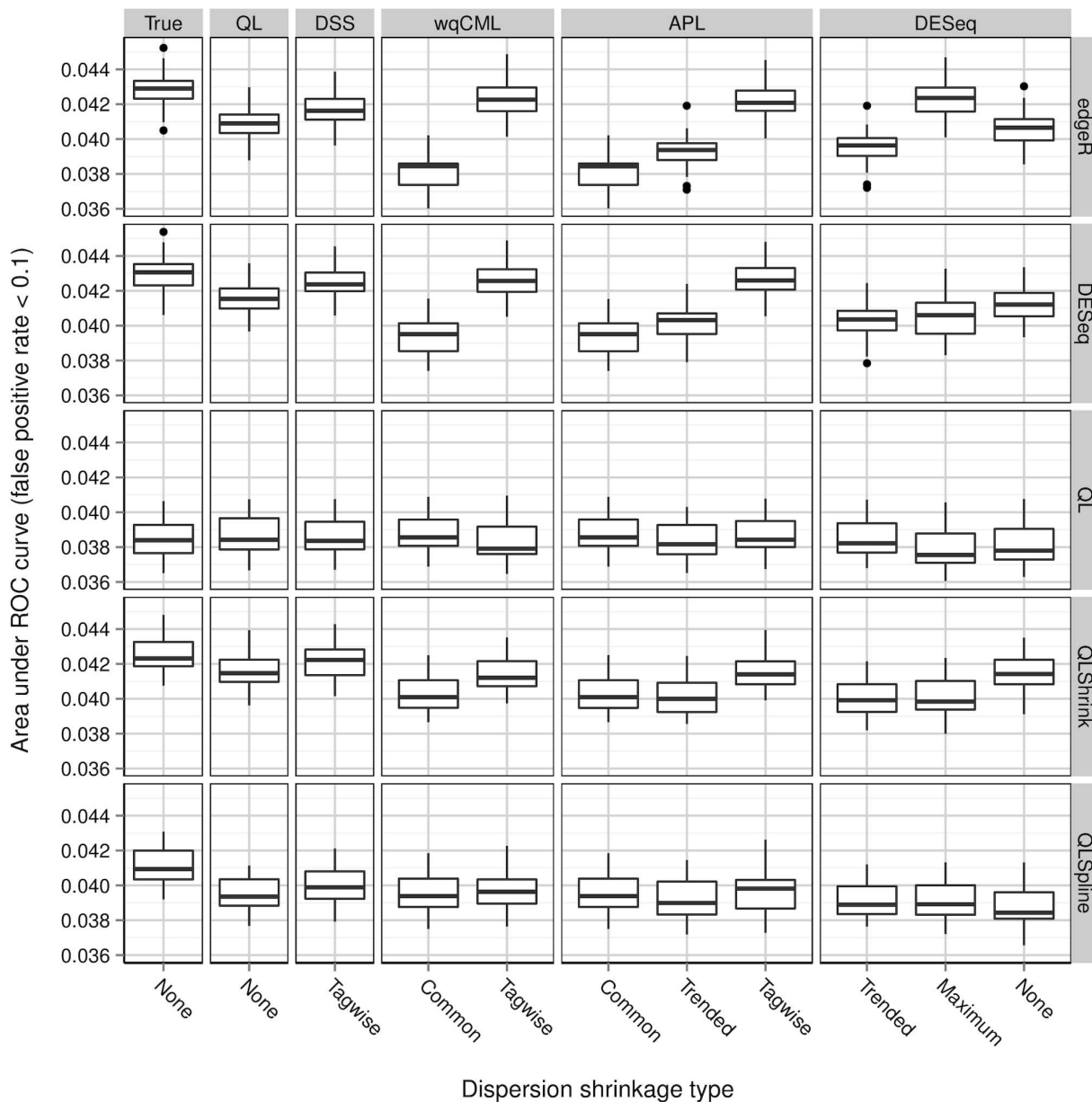
Figure 8. Simulation setting III: areas under ROC curves. Boxplots of AUC calculated based on 30 pseudo-datasets are shown for each combination of dispersion estimation method and test for differential expression. doi:10.1371/journal.pone.0081415.g008
