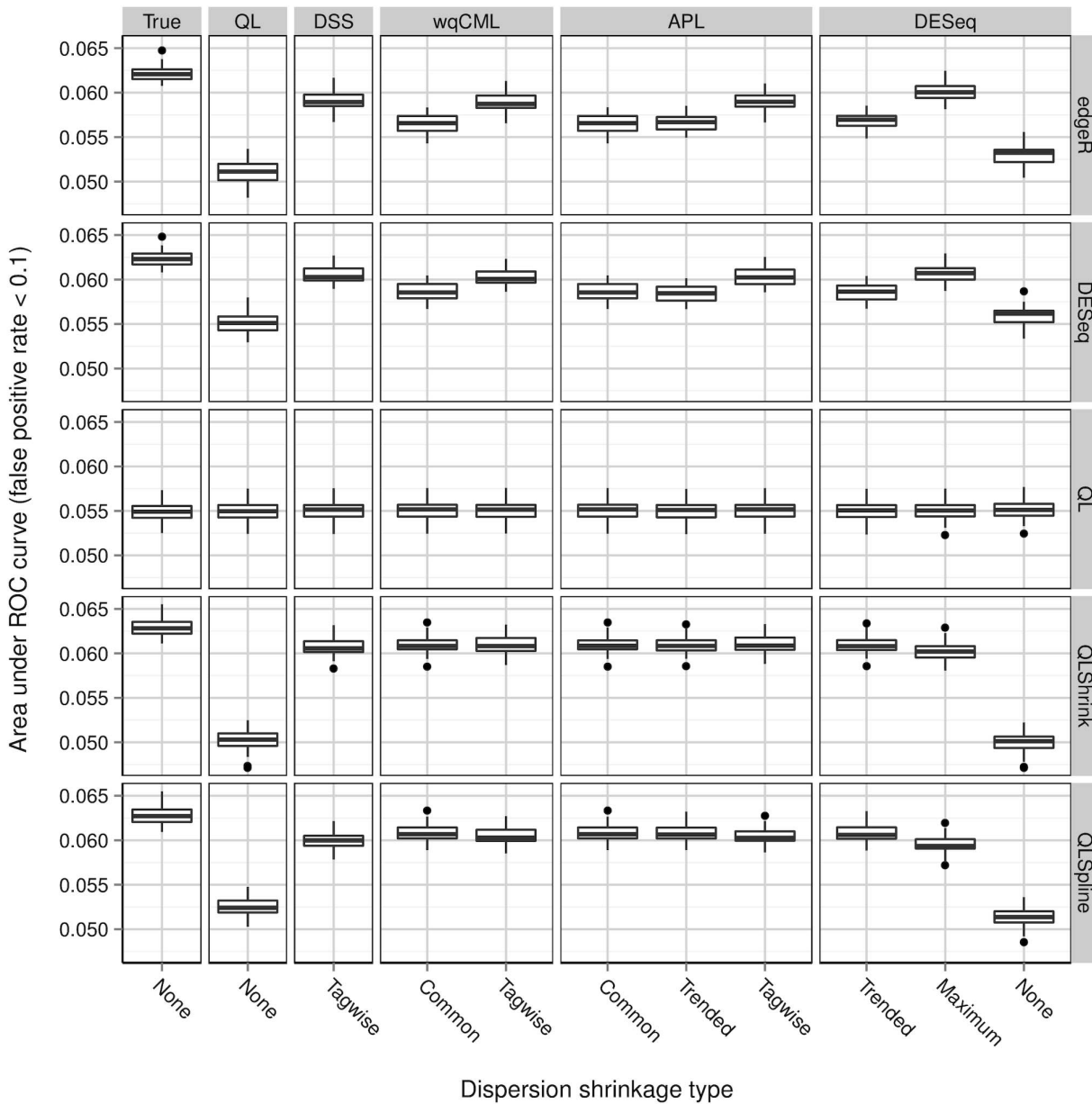
Figure 9. Simulation setting IV: areas under ROC curves. Boxplots of AUC calculated based on 30 pseudo-datasets are shown for each combination of dispersion estimation method and test for differential expression. doi:10.1371/journal.pone.0081415.g009
