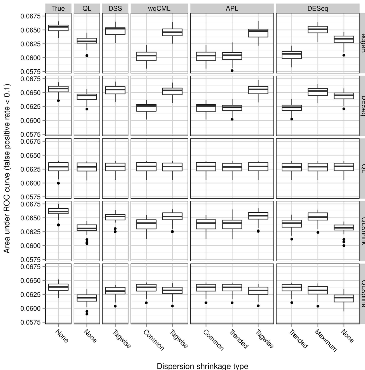
Figure 10. Simulation setting V: areas under ROC curves. Boxplots of AUC calculated based on 30 pseudo-datasets are shown for each combination of dispersion estimation method and test for differential expression. doi:10.1371/journal.pone.0081415.g010
