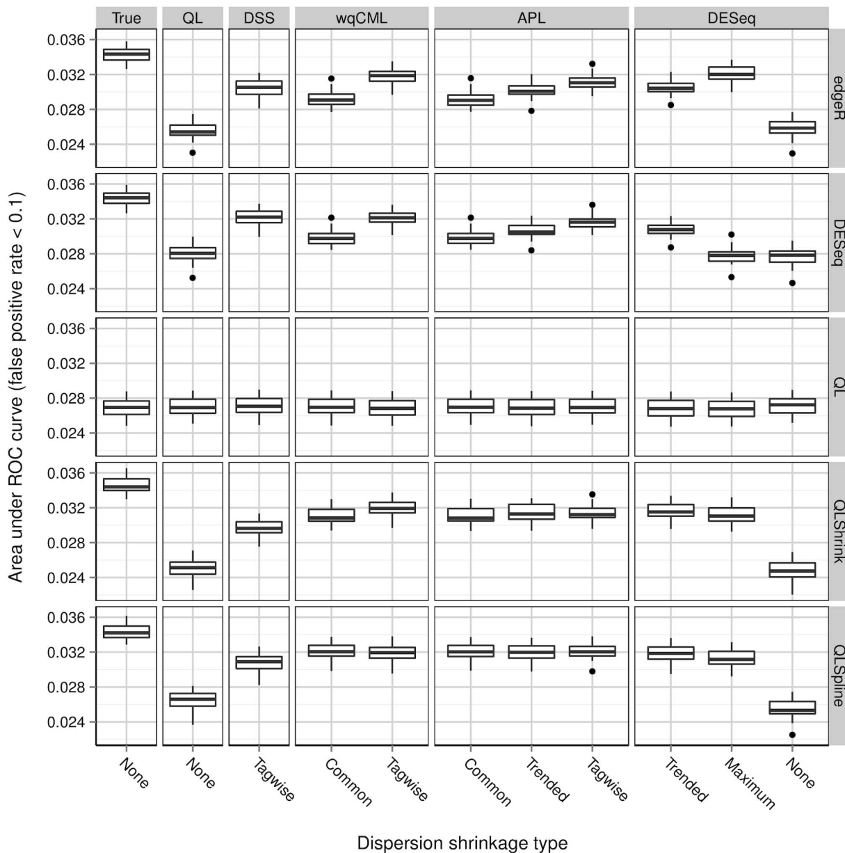
Figure 6. Simulation setting I: areas under ROC curves. Boxplots of AUC calculated based on 30 pseudo-datasets are shown for each combination of dispersion estimation method and test for differential expression. doi:10.1371/journal.pone.0081415.g006
