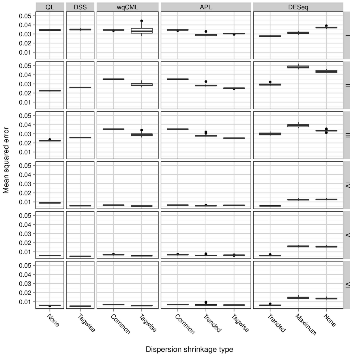
Figure 3. Mean squared error of the transformed dispersions. doi:10.1371/journal.pone.0081415.g003
