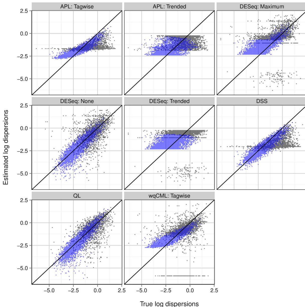
Figure 4. Simulation setting II: estimated vs true dispersions for an example pseudo-dataset. Dispersions with gene-wise log geometric mean counts below the median (log mean from -2.17 to 1.63 ) are shown in black, while those above the median (log mean from 1.63 to 10.6 ) are shown in light blue. Overlapping points are shown in dark blue. Results for simulation settings I and III are similar. doi:10.1371/journal.pone.0081415.g004
