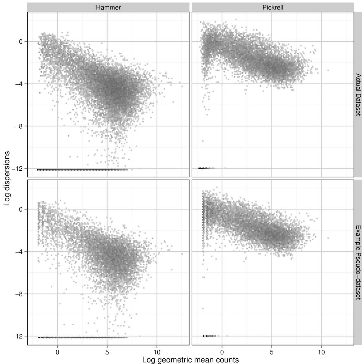
Figure 2. Dispersion-mean relationships. The top two panels show the relationship between the log QL-method-estimated dispersions and the gene-wise log geometric mean counts of the Hammer and Pickrell datasets. The bottom two plot the analogous quantities for example simulated pseudo-datasets, except that the log dispersions plotted are the true log dispersions used to simulate the pseudo-counts (i.e., the b_g 's) and the gene-wise log geometric mean counts are the a_g 's used in the simulations. Bins in these two-dimensional histograms are shaded by their log frequency. doi:10.1371/journal.pone.0081415.g002
