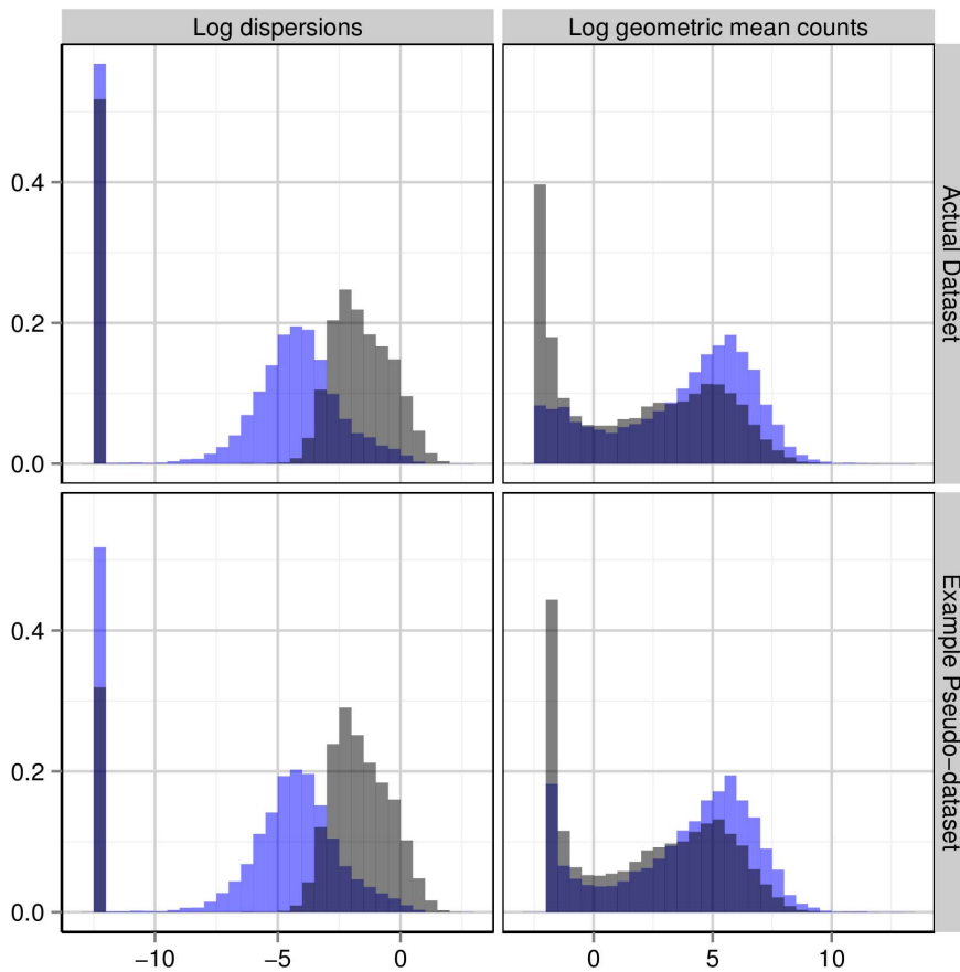
Figure 1. A look at the data. Hammer data and Hammer-generated pseudo-data are in blue, while Pickrell data and Pickrell-generated pseudo-data are shown in black. The top two panels show the gene-wise log geometric mean counts and log dispersion estimates, estimated with the QL method, for the Hammer and Pickrell datasets. The bottom two panels plot the analogous quantities for example simulated pseudo-datasets, except that the log dispersions plotted are the true dispersions used to simulate the pseudo-counts and the gene-wise log geometric mean counts are the a_g 's (log geometric mean counts from the real data) used in the simulations. The vertical bar at around -12 in the plots of the log dispersions is an artifact of the QL method, which sets extremely low dispersions (i.e., dispersions of non-overdispersed genes) to a common minimum value. doi:10.1371/journal.pone.0081415.g001
