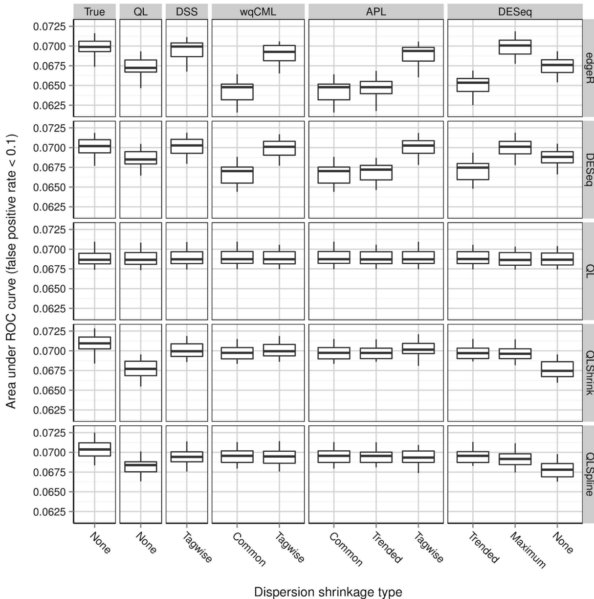
Figure 11. Simulation setting VI: areas under ROC curves. Boxplots of AUC calculated based on 30 pseudo-datasets are shown for each combination of dispersion estimation method and test for differential expression. doi:10.1371/journal.pone.0081415.g011
