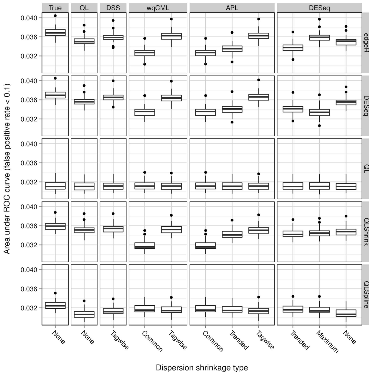
Figure 7. Simulation setting II: areas under ROC curves. Boxplots of AUC calculated based on 30 pseudo-datasets are shown for each combination of dispersion estimation method and test for differential expression. doi:10.1371/journal.pone.0081415.g007
