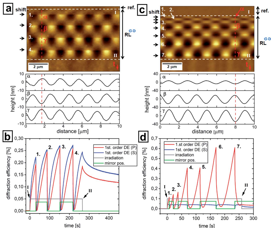
Fig. 5 (a) In situ recorded AFM micrograph of the Pazo polymer film ( h_{\text{Pazo}} = 1 \mu\text{m} ) during irradiation with RL IP ( \lambda = 491 \text{ nm} , I = 200 \text{ mW cm}^{-2} ; \Lambda = 2 \mu\text{m} ). The interference pattern is shifted four times by \lambda/2 of the optical period each after 60 s of irradiation. After each shifting of the IP the initial SRG is erased and a new SRG is formed with interchanged position of topography maxima and minima. The irradiation was stopped at the point where the surface was flat again, marked by dashed white line (II). (b) The evaluation of the 1 st order DE recorded in plane (red curve) and out-of-plane (blue curve) is presented as a function of time for four successive IP shifts. A drastic drop in the diffraction efficiency became noticeable whenever the interference pattern is shifted. (c) AFM micrograph of poly(MMA-co-DR1A) film topography ( h_{\text{poly(MMA-co-DR1A)}} = 600 \text{ nm} ) irradiated with periodically shifted RL IP with continuously increasing irradiation time: 7 s, 14 s, 17 s, 32 s, 44 s, 56 s, 65 s. (d) The corresponding 1 st order DE recorded simultaneously with the topography change in (c). Red line in (a) and (c) indicates the direction along which the cross-section was recorded as indicated in the corresponding plots below (a) and (c).
