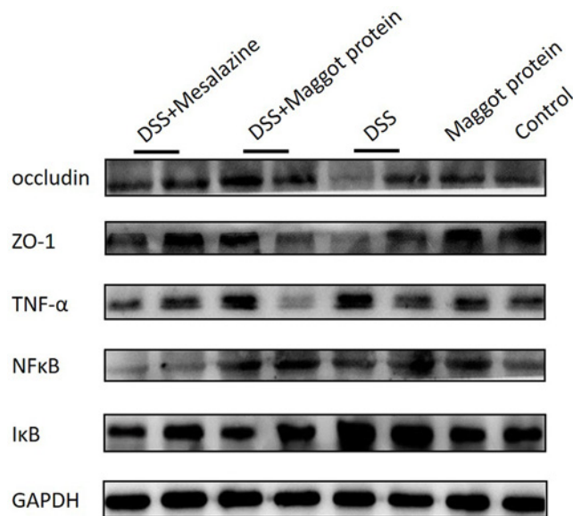
Figure 4. Effects of the maggot protein on the expression of the tight junction proteins and the activation of the NF \kappa B signaling pathway in DSS-induced mouse colitis
