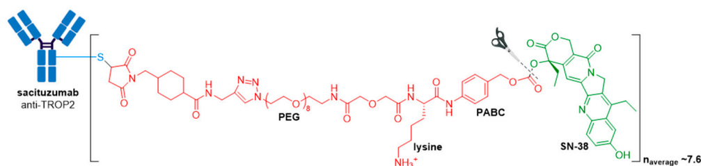
Figure 12. Structure of Trodelvy® (sacituzumab govitecan-hziy). The antibody is shown in blue, and chemical structures for linker and payload are in red and green, respectively. PEG, polyethyleneglycol.
