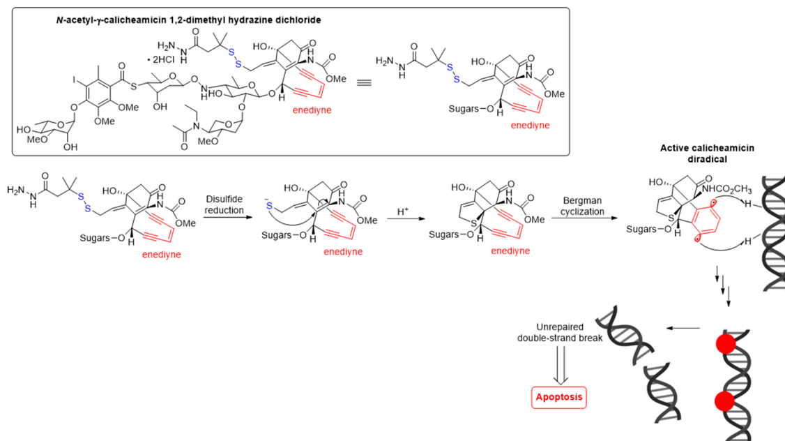
Figure 5. Mechanism for double-strand (ds) DNA cleavage by N -acetyl- \gamma -calicheamicin. The enediyne warhead is shown in red.
