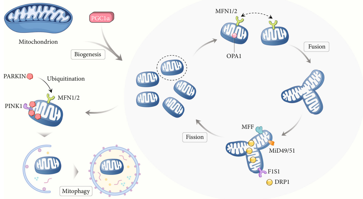
FIGURE 1: Mitochondrial dynamics. Mitochondrial dynamics includes the process of mitochondrial biogenesis, fusion, fission, and mitophagy and determine the proper abundance and function of mitochondria. (1) PGC-1 \alpha regulates mitobiogenesis and initiates mtDNA transcription through its downstream factors, such as NRF1/2. (2) Mitofusion 1/2(MFN1/2) on the outer mitochondrial membrane and optic atrophy 1 (OPA1) on the inner mitochondrial membrane regulates mitochondrial fusion. (3) DRP1 serves to constrict mitochondrion physically and uses FIS1 as mitochondrial targets to form the fission complex, and MFF and MiD49/51 also participate in mitochondrial fission. (4) Canonical regulation of mitophagy includes the PINK1/PARKIN pathway; PINK1 recruits PARKIN on mitochondrion where PARKIN ubiquitinates downstream proteins and initiates the form of mitophagy.
