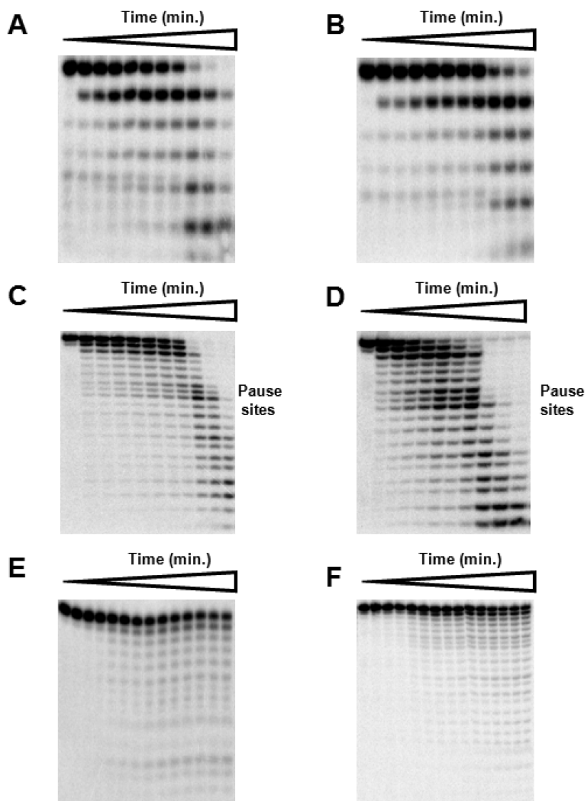
Figure 2. Distributive removal of UL30 exonuclease by nucleotides. UL30 or UL30–UL42 was incubated with DNA ( 1\ \mu\text{M} ) and aliquots were taken out at various times. (A) Phosphorimages of the products of DNA 15SS degradation using UL30–UL42. (B) Phosphorimages of the products of DNA 15SS degradation using UL30. (C) Phosphorimages of the products of DNA 35SS degradation using UL30–UL42. (D) Phosphorimages of the products of DNA 35SS degradation using UL30. The time points for legends (A)–(D) were 0, 0.25, 0.5, 0.75, 1, 1.25, 1.5, 2, 5, 7, and 10 min. (E) Phosphorimages of the products of DNA 35C degradation using UL30–UL42 at time intervals 0, 0.5, 1, 2, 5, 7, 10, 15, 20, 25, 30, 40, 50, and 60 min. (F) Phosphorimages of the products of DNA 35C degradation using UL30 at time intervals 0, 0.25, 0.5, 1, 2, 5, 7, 10, 15, 20, 25, 30, 40, 50, and 60 min. Note: The gels shown are representative of experiments that were performed multiple times.
