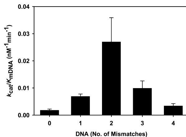
Figure 1. Exonuclease assays using 15/33 mer duplex DNA containing 0–4 mismatches at the primer terminus ( \text{DNA}_{15\text{C}} , \text{DNA}_{15\text{TG}} , \text{DNA}_{2\text{MM}} , \text{DNA}_{3\text{MM}} , and \text{DNA}_{4\text{MM}} ). Plot of k_{\text{cat}}/K_{\text{mDNA}} as a function of the number of mismatches present at the primer terminus.
