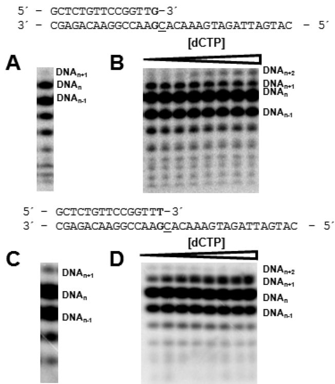
Figure 3. Translocation of DNA 15GG and DNA 15TG between polymerase and exonuclease sites. UL30 was incubated with primer–template (1 μM) in the presence of either 100 μM dGTP or 100 μM dGTP and varying concentrations of dCTP, the next correct incoming nucleotide. Reactions were quenched after 5 min and reaction products were separated by denaturing gel electrophoresis. The sequences of DNAs containing G/G and T/G mismatches are shown. (A) Phosphorimage of the products of DNA extension and degradation using 100 μM dGTP and DNA containing a G/G mismatch (DNA 15GG ). (B) Phosphorimages of the products of DNA 15GG extension and degradation using varying dCTP concentrations (5, 10, 50, 100, 200, 400, 800, and 2000 μM) and dGTP at 100 μM. (C) Phosphorimage of the products of DNA extension and degradation with UL30 using 100 μM dGTP and DNA containing a T/G mismatch (DNA 15TG ). (D) Phosphorimages of the products of DNA 15TG extension and degradation using varying dCTP concentrations (5, 10, 50, 100, 200, 400, 800, and 2000 μM) and dGTP at 100 μM.
