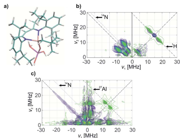
Fig. 5 (a) Model for 1@Al_2O_{3-700} species representing a neutral [(Al_5O)Ti(nacnac)(CH_2^tBu)] complex based on agreement with HYSORE spectra. (b) X-band HYSORE spectrum of 1@Al_2O_{3-700} (blue) and simulation (green), based on DFT calculations on the obtained model. (c) Q-band HYSORE spectrum of 1@Al_2O_{3-700} (blue) and simulation (green), based on DFT computed EPR parameters from the obtained model (a) for ^{14}N , combined with EPR parameters for ^{27}Al , obtained from a least squares fit of the experimental spectrum. The ridge on the anti-diagonal in the left quadrant is due to an echo crossing that was not fully suppressed by phase cycling.
