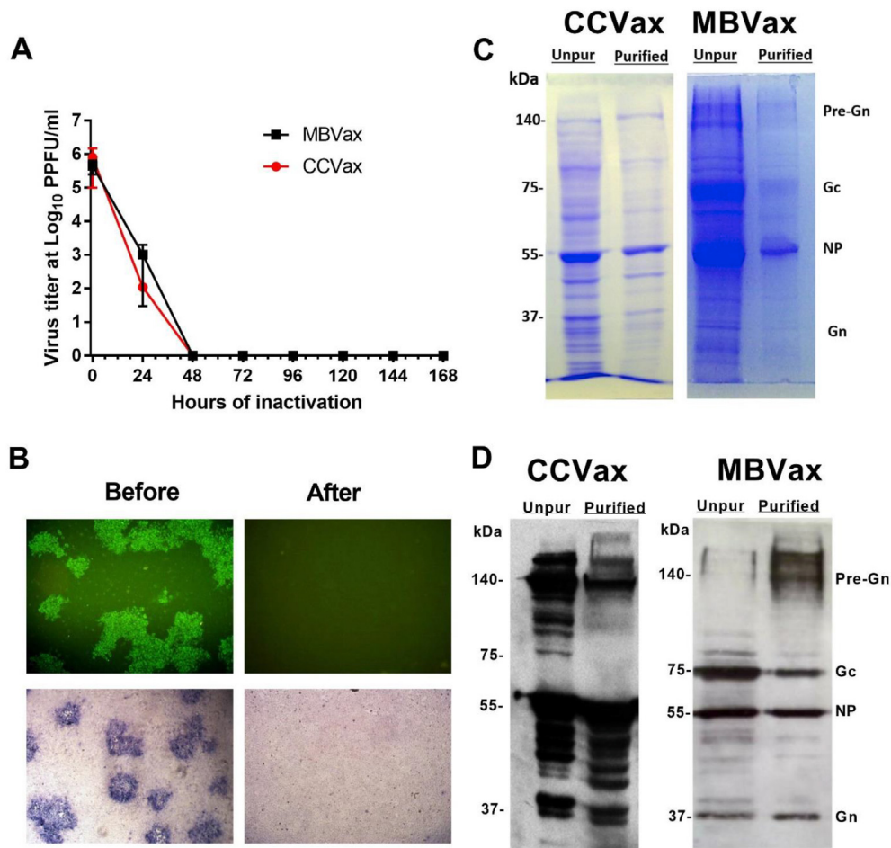
Figure 5. Inactivation of Turkey-Kelkit06 virus' infectivity by formalin (A), in Vero E6 cells, as determined by a fluorescent focus and pseudo-plaque formation assay, before and after formalin inactivation (B). SDS-PAGE (C) and Western blotting (D) analyses were performed for the CCVax and MBVax candidates to reveal protein purification and conformations (Gn, 37kDa; NP, 55 kDa; Gc, 75 kDa; Pre-Gn, 140 kDa).
