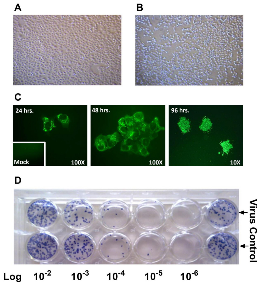
Figure 2. Characterization of Turkey-Kelkit06 virus growth in Vero E6 cells. Vero E6 cells (A) were infected with CCHFV, and the cells showed lysis and detachment from the bottom of the cell culture flasks at 5 dpi (B). Fluorescent focus analysis confirmed that virus-infected cells showed kinetic growth, and the focus sizes became larger over time (C). A 24-well plate demonstrating virus titers increasing logarithmically (Log 10) in a PFU assay after the addition of NBT substrate (D).
