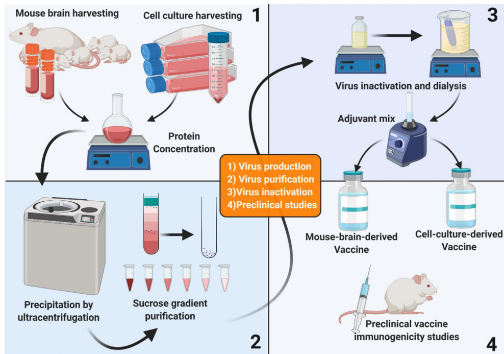
Figure 1. Study design and graphical abstract of the inactivated CCHFV vaccine platform.
