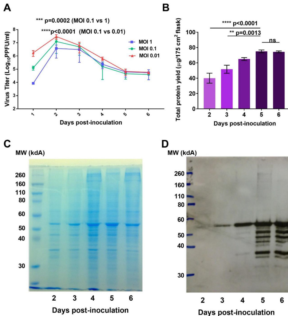
Figure 3. Optimization of Turkey-Kelkit06 viral growth and kinetics in Vero E6 cells. Cells were infected with three (1, 0.1, and 0.01) MOIs, and viral titers were measured at different time points (A). Total protein quantification by the Lowry assay, showing the daily total protein yield per infected ( 175\text{ cm}^2 ) flask (B). Viral protein analysis was performed by SDS-PAGE (C) and Western blotting (D) for CCVax candidate production in Vero E6 cells (Gn, 37 kDa; NP, 55 kDa).
