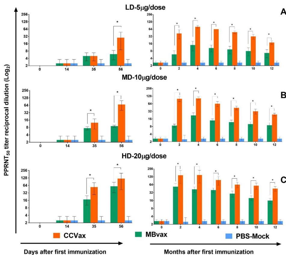
Figure 7. PPRNT 50 titers were assessed in serum samples obtained after and during immunization. Vaccine formulations of CCVax and MBVax were compared, including HD (A), MD (B), and LD (C). PPRNT 50 titers were calculated on the basis of the results obtained from a 50% reduction in the virus titer from before immunization in each mouse. The error bars show the standard errors of the mean. The two-way ANOVA comparison test was performed to assess the significance of each dose formulation (* p < 0.05).
