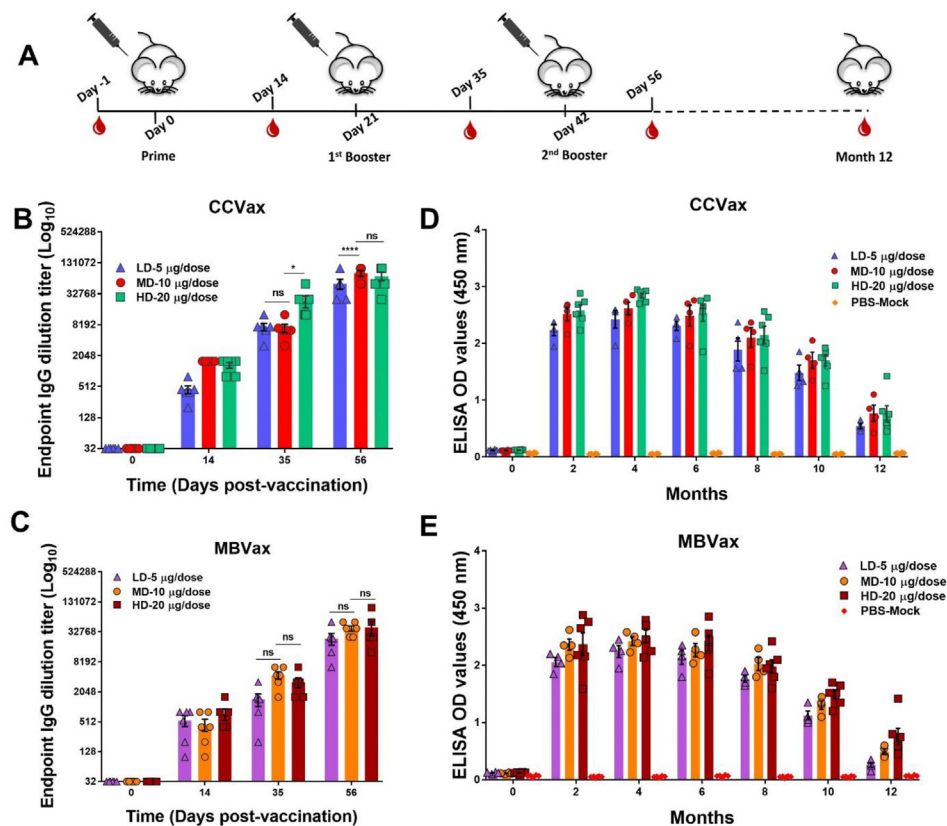
Figure 6. Vaccine schedule and vaccine-induced IgG titers in BALB/c animals. The immunization schedule was three injections at 3-week intervals, and serum samples were collected from mice before and after each immunization, and then every 2 months after the last serum samples were collected following the booster (A). Indirect ELISA measuring the Turkey-Kelkit06 virus-specific IgG responses in the sera of mice ( n = 6 ) immunized with CCVax and MBVax formulations (B and C). Evaluation of the OD of the serum IgG titer; values were measured for 1 year for both CCVax (D) and MBVax candidate recipients (E). The error bars indicate the standard deviations. The two-way ANOVA comparison test was performed to measure the significance of each dose formulation (* p < 0.05 , **** p < 0.0001 , and ns: not significant).
