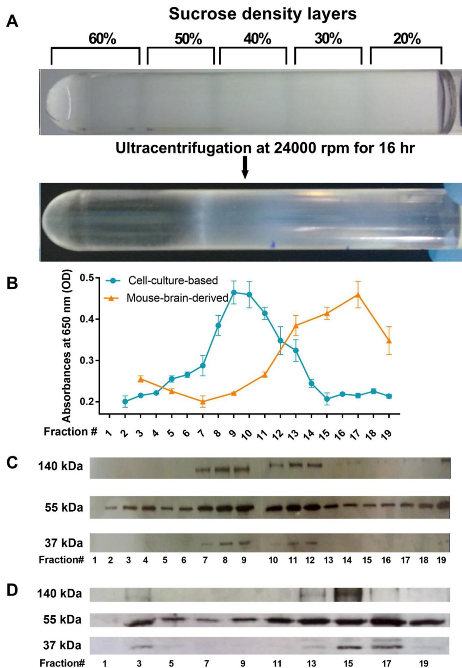
Figure 4. Separation and purification of virus particles through a discontinuous sucrose gradient ultracentrifugation. Sucrose gradient layers were overlaid on each other from 60% to 20% in SW41 ultraclear tubes, and virus suspensions were loaded on top of the gradient layers (A). Viral antigens were centrifuged through the gradient layers and fractionated to smaller volumes. Fractions were tested for protein quantification, and OD values at 650 nm absorbance were obtained (B); viral particle localizations were visualized in the cell-culture- (C) and mouse-brain-derived (D) fractions (Gn, 37kDa; NP, 55 kDa; Gc, 75 kDa; Pre-Gn, 140 kDa).
