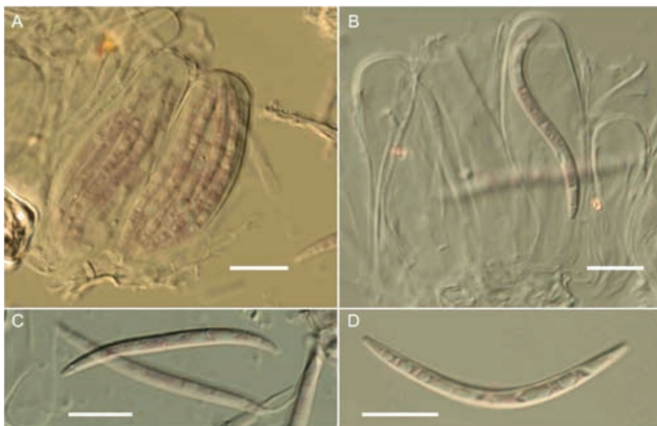
Fig. 4. Claviradulomyces xylopiei asci and ascospores (VIC 31417 mounted in lactofuchsin). A. Mature asci containing parallel to somewhat spirally arranged ascospores. B. Single vermiform ascospore within ascus. C, D. Ascospores. Bars: A = 40 µm; B = 35 µm; C = 10 µm; D = 10 µm.
