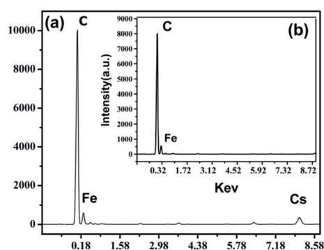
Fig. 4 EDS spectra of the unleached MMWCNTs@Cs(I)-IIP (a) and the leached MMWCNTs@Cs(I)-IIP (b).
