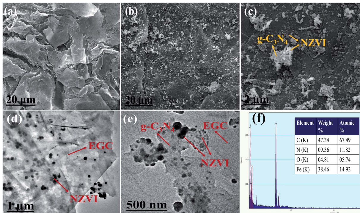
Fig. 1 SEM images of (a) EG, (b and c) NZVI/g-C 3 N 4 @EGC; TEM images of (d and e) NZVI/g-C 3 N 4 @EGC; (f) EDS spectrum of NZVI/g-C 3 N 4 @EGC.
