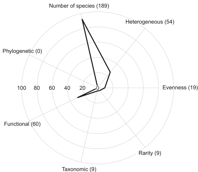
Figure 1. Assessing coral reef fish diversity. Relative importance of the main diversity components assessed in the set of the 205 papers reviewed in this study. Radar plot shows the percentage of publications assessing each diversity component. The corresponding number of papers is given in brackets. Heterogeneous indices that mix two components (number of species and equitability) are also displayed because of their popularity.
