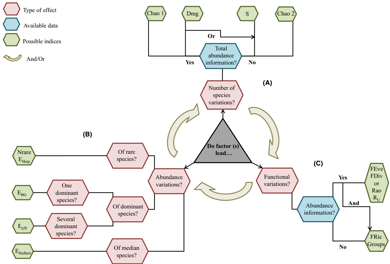
Figure 3. Flowchart providing an illustration of the use of alternatives indices. It reads from the inside outwards. A, B, and C are linked to the three paragraphs of the second part of the paper. The references, formula, and R packages of the indices mentioned are given in Appendix S2.
