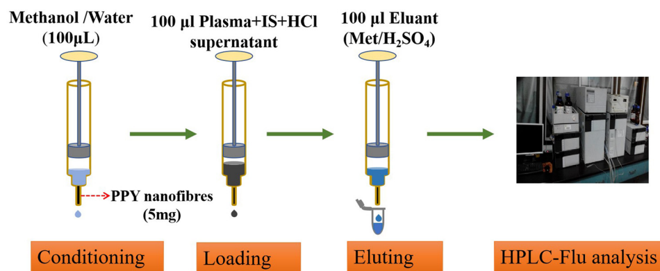
Figure S3: Schematic flow chart of PFSPE procedure for the determination of tryptophan metabolites in plasma.
