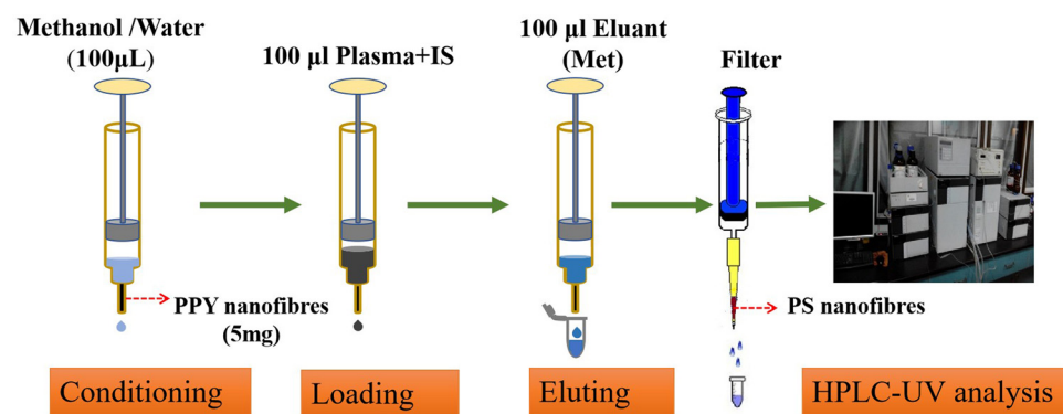
Figure S1: Schematic flow chart of PFSPE procedure for the determination of cortisol and cortisone in plasma.
