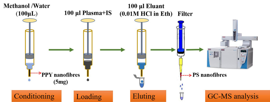
Figure S2: Schematic flow chart of PFSPE procedure for the determination of SCFAs in plasma.
