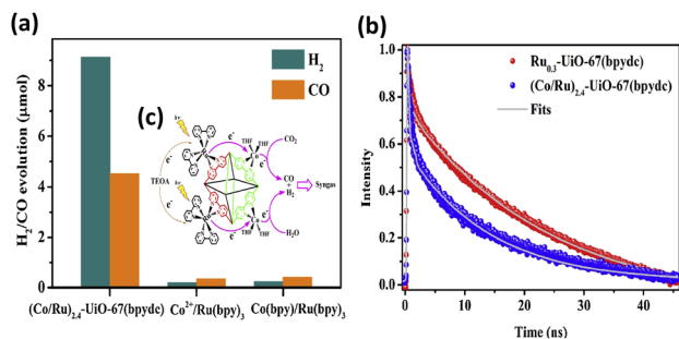
Fig. 2 (a) Results of photocatalytic \text{CO}_2 reduction under visible light illumination over (\text{Co}/\text{Ru})_{2.4}\text{-UiO-67}(\text{bpydc}) and the corresponding homogeneous counterparts. (b) Time-resolved PL spectra of (\text{Co}/\text{Ru})_{2.4}\text{-UiO-67}(\text{bpydc}) and \text{Ru}_{0.3}\text{-UiO-67}(\text{bpydc}) . Excitation and emission wavelength were 450 nm and 700 nm, respectively. (c) Proposed mechanism of interfacial charge transfer. Reproduced with permission from ref. 38. Copyright 2019, Elsevier.
