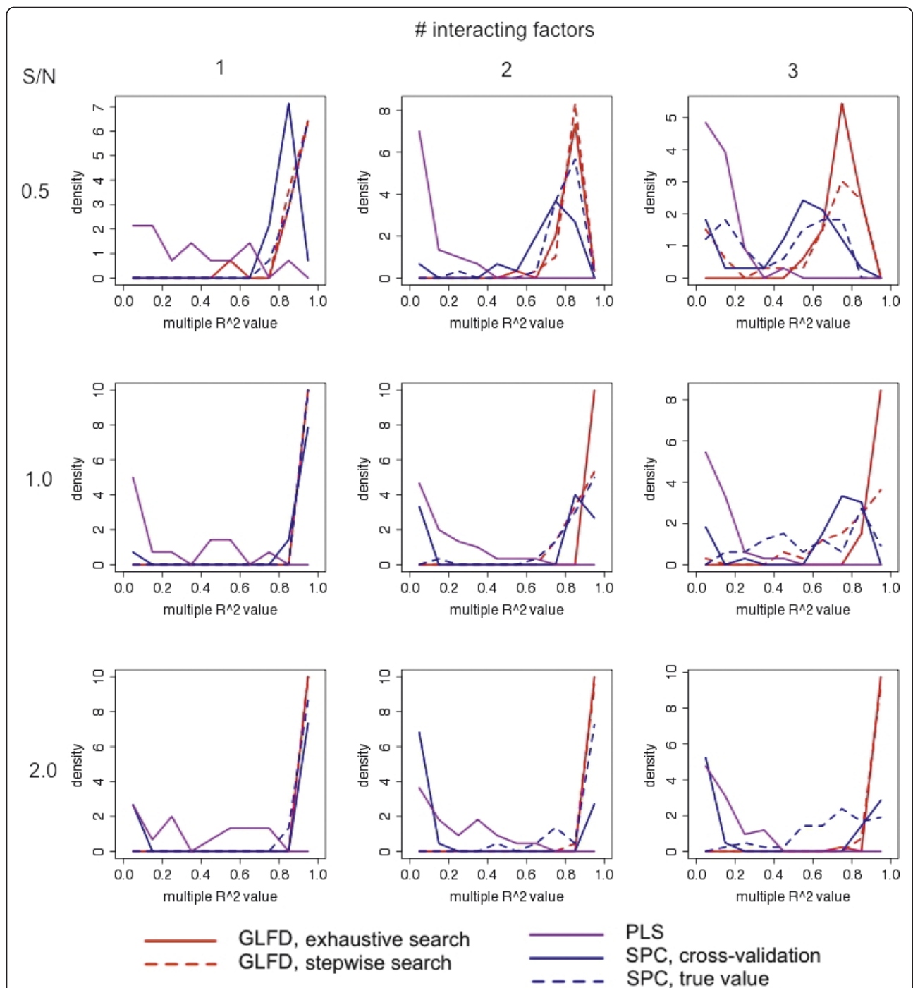
Figure 1 Simulation results showing the capability of GLFD to discover latent factors, as compared with PLS and SPC. In every simulation, 5 modules, each consisting of 200 simulated genes, were generated. The first module was governed by the clinical factor, together with 1~3 other latent factors (columns). The other four modules were governed by 2~4 factors. All factor scores were drawn independently from the standard normal distribution. Gaussian random noise was added to achieve different signal to noise ratios (rows). An additional 1000 pure noise genes were generated from the standard normal distribution. Each simulation setting was repeated 100 times. The success of latent factor recovery was evaluated by the R^2 values obtained by the regression of each latent factor against the identified factors. The relative frequencies (10 equal-sized bins between 0 and 1, equivalent to the histogram) of the R^2 values are plotted.
