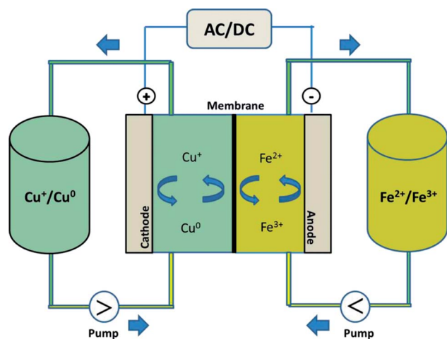
Fig. 1 Schematic illustration of the experimental set-up of a Fe/Cu redox flow battery.
