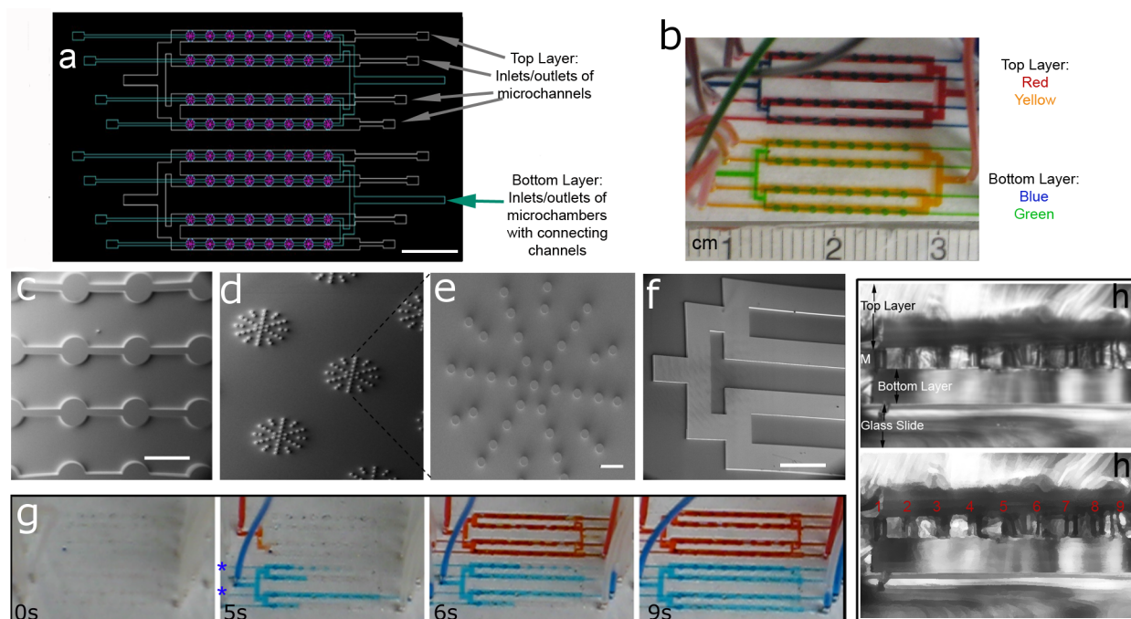
Figure 2. Design and fabrication of 3D microfluidic cell arrays. (a) AutoCAD device mask drawing of merged layers, scale bar is 2 mm; (b) top view of a 3D \mu FCA with a solid/nonpermeable PDMS middle layer, features dyed with blue and green food colors are in the bottom while red and yellow channels are in the top layer; SEM images of silicon etched masters of (c) bottom (scale bar is 1 mm), (d) middle, and (f) upper layers (scale bar is 1 mm); (e) SEM image of the enlarged middle layer; master scale bar is 100 \mu m; (g) frames of a video showing diffusion of food dyes from top to bottom layers through the middle filter layer in 5 s (two blue stars [*] point to two channels on the bottom which become blue due to dye diffusion from the top); side-view of one unit of 3D microfluidic cell arrays ( \mu FCA) captured under a 5 \times phase contrast objective showing (h 1 ) three PDMS layers bonded on a glass slide (“M” indicates the middle PDMS layer with clustered pores) and (h 2 ) numbered pores in the middle layer in a dry brush processed image using Photoshop.
