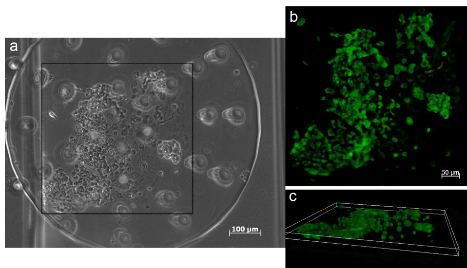
Figure 3. Lung cancer cells with long fluorescence trackers encapsulated in hydrogel and cultured in a chamber of a 3D \mu FCA for 15 days, (a) phase contrast image, (b) 2D projected image after deconvolution of fluorescence z-stack images, and (c) 3D view of (b), where its dimension is 550 \times 500 \times 70 \mu\text{m} in x (length from left to right), y (depth), and z (thickness from bottom to top) directions.
