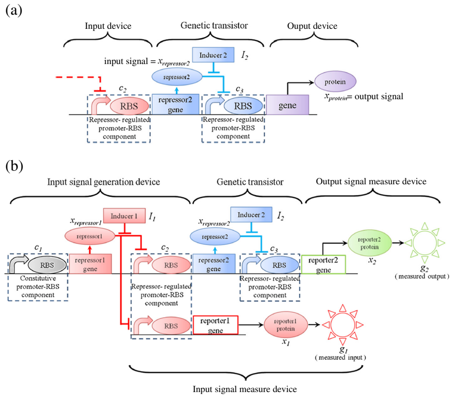
Figure 1 The representation of synthetic genetic transistor circuit. (a) A genetic transistor. (b) A genetic transistor with measurement circuit. The input signal of the genetic transistor is measured by RFP reporter and the output signal of the genetic transistor is measured by GFP reporter.
