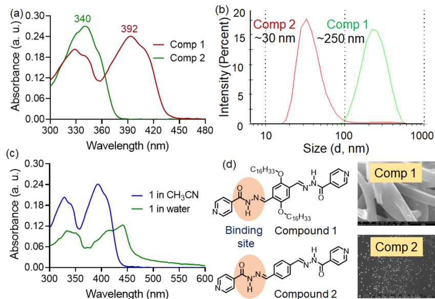
Fig. 1 (a) UV-visible spectra of 1 and 2 (10 \mu M) in CH 3 CN–water (7 : 3) medium. (b) Dynamic light scattering experiment of 1 and 2 (10 \mu M) in CH 3 CN–water (7 : 3) medium. (c) UV-visible spectra of 1 (10 \mu M) in water and CH 3 CN medium. (d) FESEM images and structure of compound 1 and 2.
