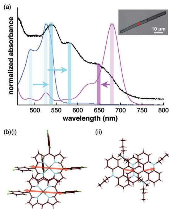
Fig. 13 (a) UV/vis absorption spectrum of the single crystal of 2\text{ni}^- - \text{TATA}^+ (black) along with those of the solution states ( 1 \times 10^{-5} M in \text{CH}_2\text{Cl}_2 ) of 2\text{ni}^- - \text{TBA}^+ (magenta) and \text{TATA}^+ - \text{Cl}^- (cyan) (inset: optical microscopy image of a single crystal of 2\text{ni}^- - \text{TATA}^+ with the red spot indicating the position where UV/vis absorption measurement was conducted) and (b) arrangement of transition dipole moments in the dimers of (i) 2\text{ni}^- and (ii) \text{TATA}^+ in the crystal state.
