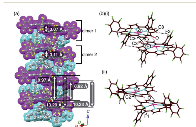
Fig. 8 Solid-state structure of 2\text{zn}^- - \text{TBA}^+ as (a) columnar structures and detailed structures of (b)(i) dimer 1 and (b)(ii) dimer 2. Distances for (b)(i): Zn⋯O = 2.10 \text{\AA} , C2(-H)⋯F1 = 3.28 \text{\AA} , C3(-H)⋯F1 = 3.30 \text{\AA} and C8(-H)⋯F2 = 3.30 \text{\AA} ; distances for (b)(ii): Zn⋯O = 2.09 \text{\AA} and C2(-H)⋯F1 = 3.36 \text{\AA} . Colour code in (a): magenta and cyan refer to anion and cation parts, respectively. Atom colour code in (b): brown, pink, cyan, red, green and magenta refer to carbon, hydrogen, nitrogen, oxygen, fluorine and zinc, respectively.
