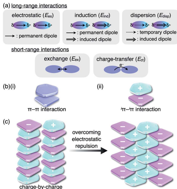
Fig. 1 (a) Fundamental intermolecular forces, (b) representative model structures based on (i) \pi - \pi and (ii) {}^i\pi - {}^i\pi interactions and (c) charge-by-charge assembly (left) and an actually observed assembly mode (right).
