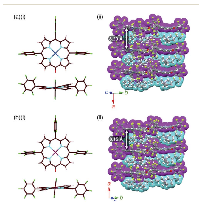
Fig. 7 Solid-state structures of (a) 2\text{pd}^- - \text{TBA}^+ and (b) 2\text{pt}^- - \text{TBA}^+ as (i) top and side views of porphyrin anions and (ii) packing structures of ion pairs. Atom colour code in (i): brown, pink, cyan, red, green, blue and purple refer to carbon, hydrogen, nitrogen, oxygen, fluorine, palladium and platinum, respectively. Colour code in (ii): magenta and cyan refer to anion and cation parts, respectively.
