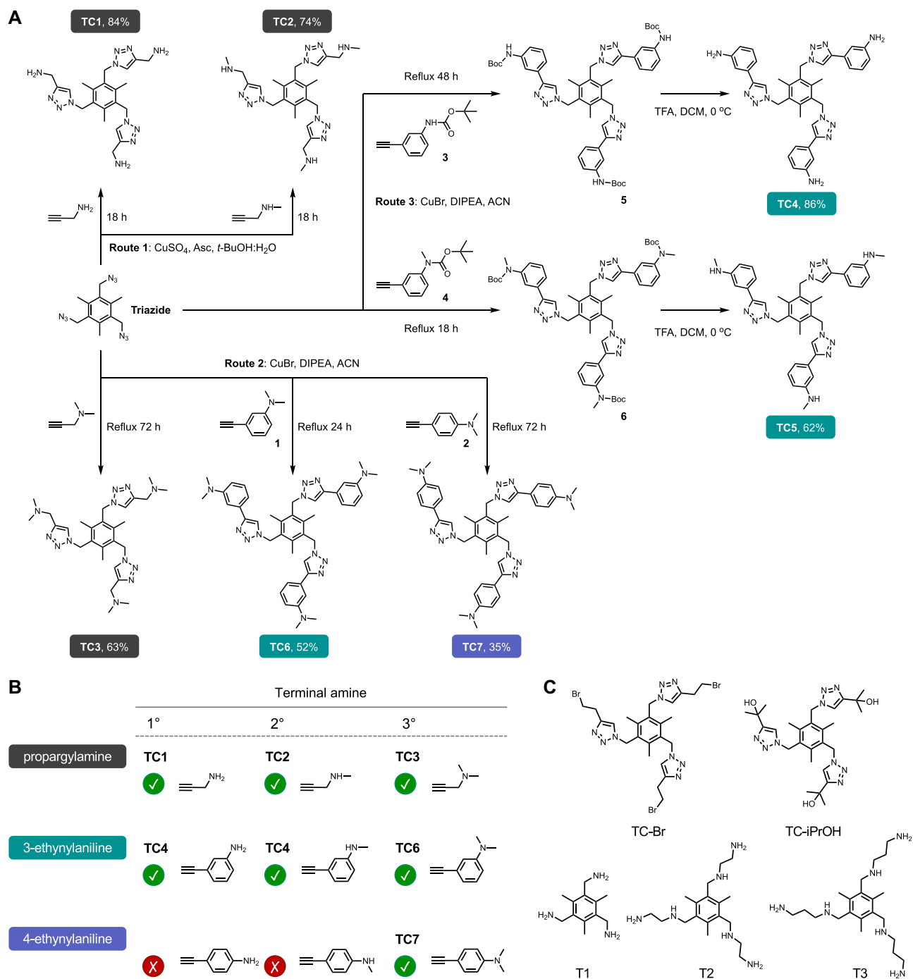
Figure 1. (A) General synthetic routes for the Tri-Click series. Route 1: alkyne functionalised primary and secondary amines were coupled to triazole using the CuAAC reaction. Route 2: tertiary amines were clicked with Cu(I). Route 3: Cu(I) click conditions of Boc-protected benzyl substituted amines followed by deprotection. (B) Structures of successful and attempted click reactions of alkyne-amines. (C) Tri-Click SAR controls. Clicked derivatives with no terminal amines TC-Br and TC- t -PrOH and simplified polyamine analogues T1-3.
