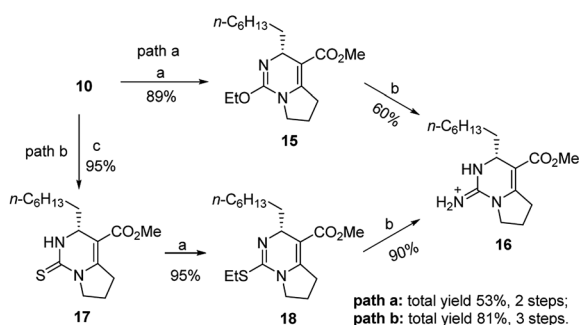
Scheme 3 Reagents and conditions: (a) Et 3 O + BF 4 – , NaHCO 3 , dry CH 2 Cl 2 , r.t., 1 h; (b) NH 4 + EtCO 2 – , 80 °C, 3 h; (c) Lawesson's reagent, xylene, 120 °C, 2 h, 95%.
