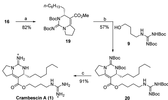
Scheme 4 Reagents and conditions: (a) NaH, dry THF, 0 °C, then DMAP, (Boc) 2 O, r.t.; (b) EtSLi, HMPA, r.t., then BOPCl, NEt 3 , dry CH 2 Cl 2 , r.t.; (c) CF 3 CO 2 H, dry CH 2 Cl 2 .
