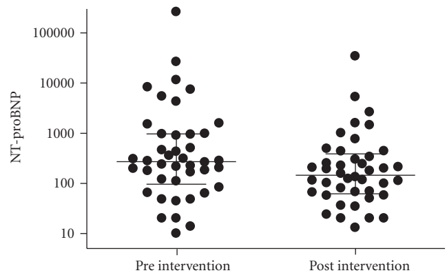
FIGURE 1: The evolution of the actual NT-proBNP values (log 10, pg/mL) before and after intervention to treat a cardiac stenosis. The difference between the values before and after intervention was highly statistically significant using Wilcoxon’s matched pairs test ( P < .0001 ).
