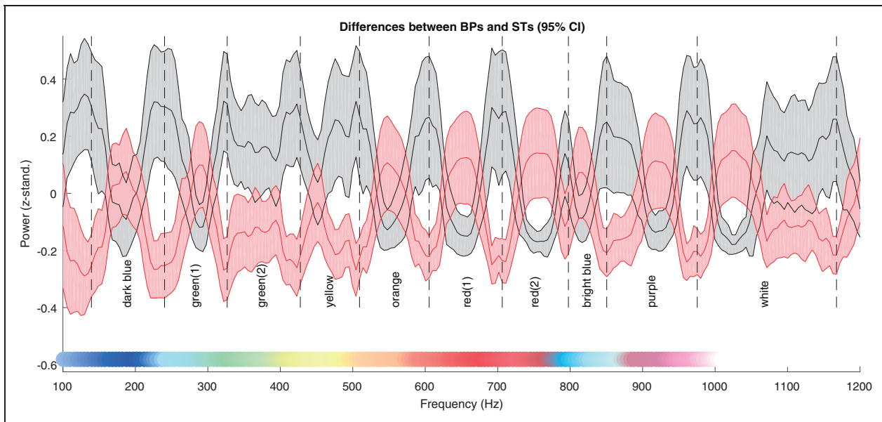
Figure 3. Group Differences (BPs Versus STs). Note. Baseline means and 95%CI for BPs (black) and STs (red).
