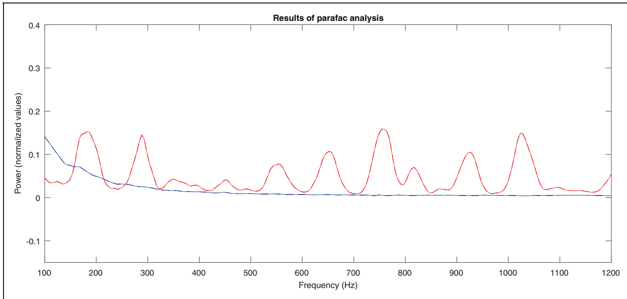
Figure 1. Results of Parafac Analysis. Note. Results from parafac analyses in the frequency domain: The first factor (blue line) represents a 1/f -factor, while the second factor (red line) contains potential biofield information. Due to the large sample size, the 95% confidence intervals (from 1000 bootstrap samples with 50% sample size of the total sample) are very tight around the mean.
