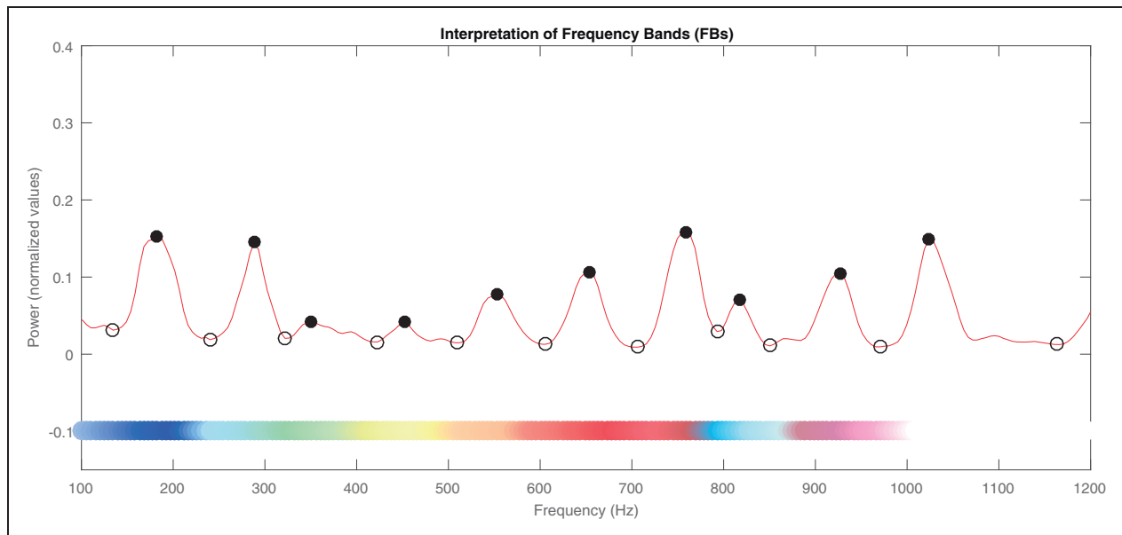
Figure 2. Interpretation of Frequency Bands (FBs). Note. Interpretation of the second factor (red line, cf. Figure 1) of parafac analysis (based on the total sample). Ten distinct peaks with their respective maxima (filled) and minima (circled) were detected. Exact values for the frequencies can be found in Table 2, respectively. For interpretation of the labeling of the newly identified FBs, the color spectrum at the bottom follows the suggestions from earlier research. 21,22
