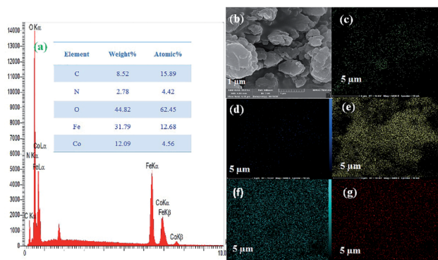
Fig. 5 EDS analysis of the N-GQDs/CoFe 2 O 4 nanocomposite (a) and surface elemental mapping-EDS of Co, Fe, O, C, and N elements (b–g).
