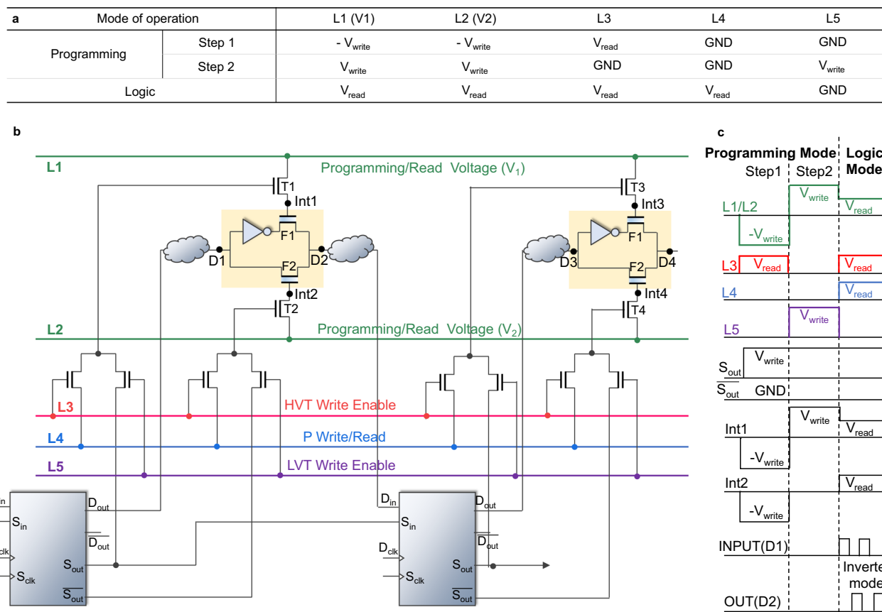
Fig. 4 Circuit description of the proposed encryption key distribution utilizing the existing data-scan flipflops in the IC. Gray bubbles indicates the functional logic. The circuits in the yellow enclosure show encryption logic. a The biasing scheme for the proposed peripheral scheme. b Schematic of the proposed encrypted IC with suggested peripheral circuitry by reusing the scan chain for the key distribution toward encryption blocks. c Peripheral biasing waveforms in the programming and logic mode operation. Note, To minimize the routing lines and periphery required, most of the metal lines are shared temporally in the operations.
