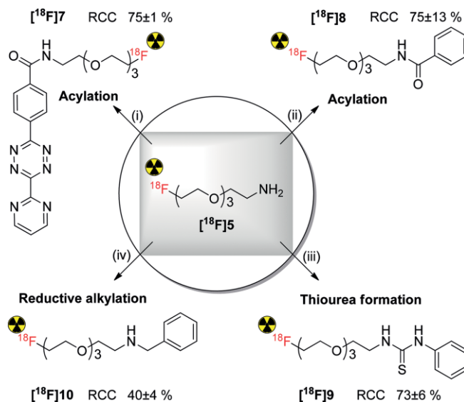
Figure 3. Versatile indirect labeling through acylation, thiourea formation and reductive alkylation using amine ^{18}\text{F} [5] as a synthon. (i) Tetrazine 6 (Supporting Information), r.t. 5 min; (ii) \text{PhCOCl} , r.t. 5 min; (iii) \text{PhNCS} , 100 °C, 5 min; (iv) \text{PhCHO} , \text{NaBH}_3\text{CN} , \text{AcOH} , 120 °C, 5 min.
