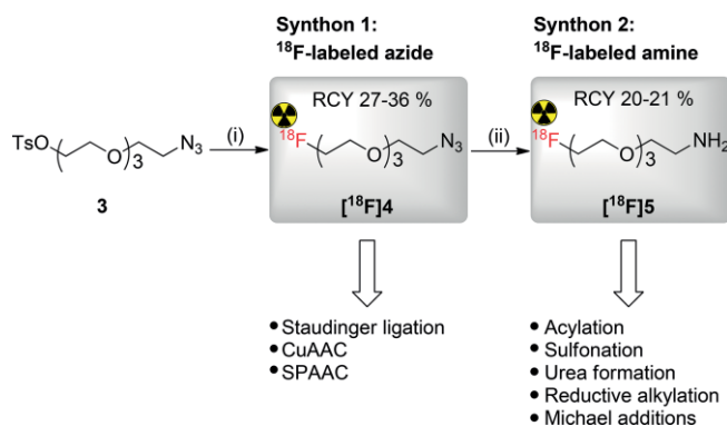
Figure 2. Two different ^{18}\text{F} -labeled synthons produced from one precursor: (i) ^{18}\text{F} KF, \text{K}_2\text{CO}_3 , \text{K}_{222} , DMSO, 120 °C, 10 min; (ii) 1. \text{PPh}_3 , MeCN, 100 °C, 10 min; 2. NaOH, 100 °C, 10 min. RCYs are decay corrected.
