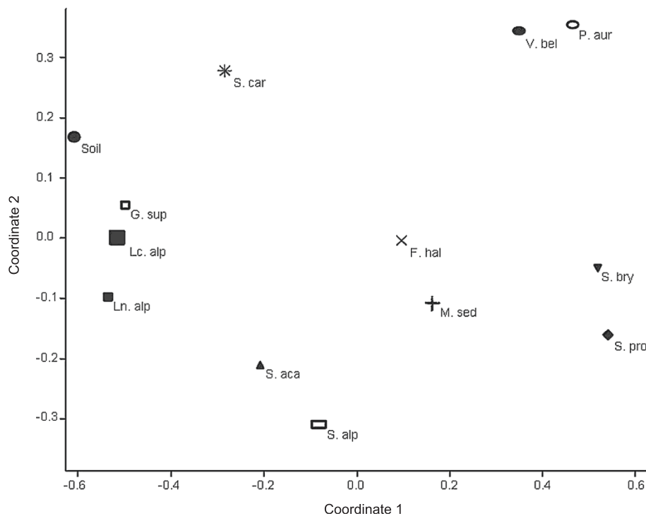
Figure 4 Distribution of plants through DGGE bacterial diversity. Non-Metric Multidimensional Scaling analysis of the 12 pioneer plants and the bare soil according to UniFrac distance matrix. Plant names are as listed in Figure 1.
