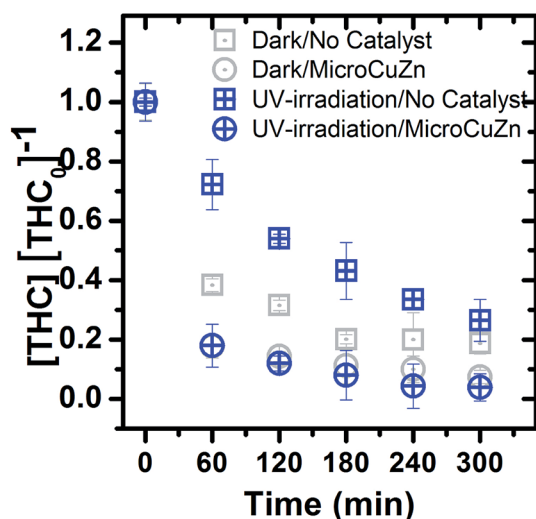
Fig. 3 THC concentration history ( 1 \mu\text{M} initial concentration at pH 7) to elucidate MicroCuZn ( 10 \text{ g L}^{-1} ) catalysis effects. Experiment were conducted at 20 \text{ }^\circ\text{C} and UV-irradiation was 9.9 \mu\text{einstein per min} .
