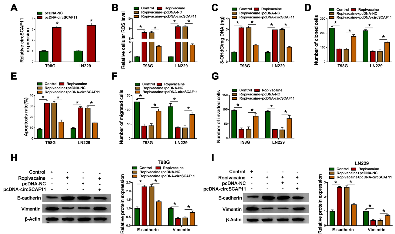
Figure 3 CircScaf11 overexpression decreases the inhibition effects of ropivacaine on glioma progression. (A) QRT-PCR results investigated that circScaf11 expression was dramatically upregulated after pcDNA-circScaf11 transfection. (B) ROS measurement assay showed the effect between ropivacaine and circScaf11 overexpression on ROS level. (C) 8-OHdG determination assay revealed the effect between ropivacaine and circScaf11 overexpression on 8-OHdG production. (D) Cell colony formation assay illustrated that circScaf11 overexpression hindered the inhibition effect of ropivacaine on cell proliferation. (E) Flow cytometry analysis showed that circScaf11 overexpression hindered the promotion effect of ropivacaine treatment on cell apoptosis. (F and G) The migration and invasion abilities of T98G and LN229 cells were detected by transwell assay. (H and I) The effects between ropivacaine and circScaf11 overexpression on E-cadherin and Vimentin protein expression were detected by Western blot. * P < 0.05 .
