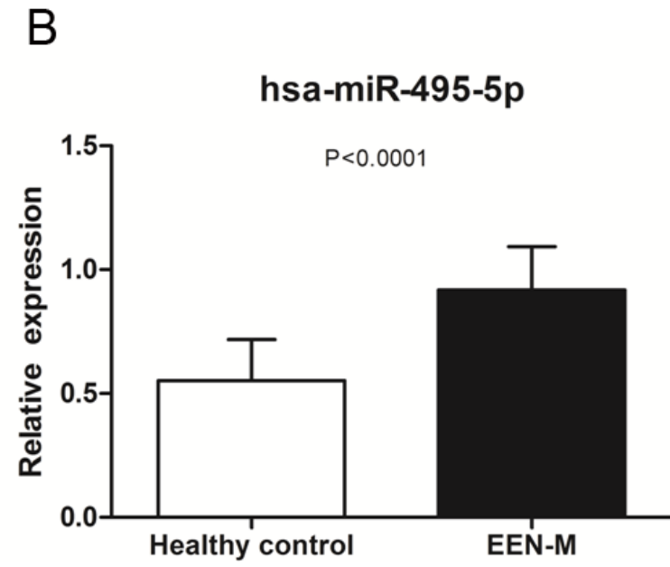
Figure 3. Comparison between EEN-M and healthy control: (A) heat map of differentially expressed miRNAs clearly separated EEN-M and normal samples; and (B) qRT-PCR validation of miRNAs differentially expressed in EEN-M.
