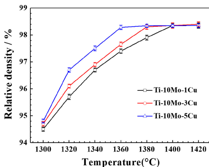
Fig. 2. Influence of sintering temperature and Cu contents on the relative density of Ti–10Mo-xCu alloy.
