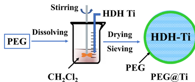
Fig. 1. Schematic illustration of the coating process of Ti powder with PEG.
