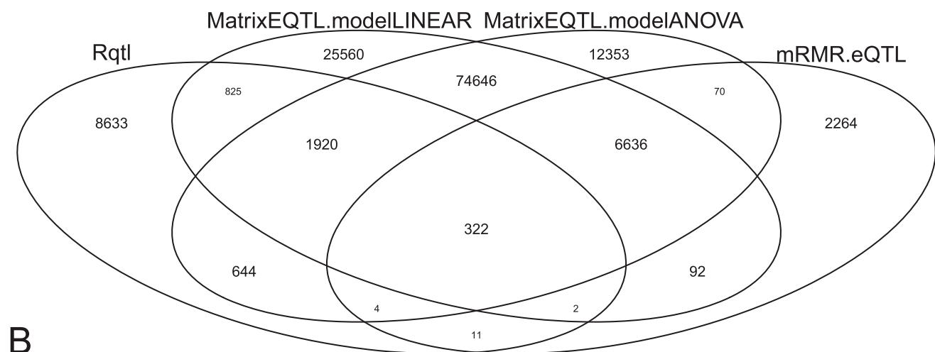
Figure 2. The venn diagram of mRMR.eQTL, R/qtl, MatrixEQTL.modelLINEAR and MatrixEQTL.modelANOVA in female and male mice. (A) The venn diagram of mRMR.eQTL, R/qtl, MatrixEQTL.modelLINEAR and MatrixEQTL.modelANOVA in female mice; (B) The venn diagram of mRMR.eQTL, R/qtl, MatrixEQTL.modelLINEAR and MatrixEQTL.modelANOVA in male mice. doi:10.1371/journal.pone.0067899.g002
