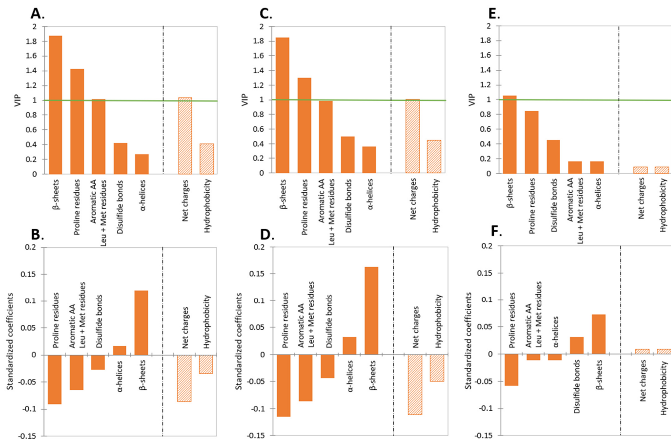
Figure 4. (A,B) The overall (i.e., for intact + restructured proteins) comparison and importance of the impact of the structural components of proteins on the pepsinolysis. (C,D) Protein in intact forms (groups ‘native’ and ‘milk’). (E,F) Proteins are in restructured forms (groups ‘gel’ and ‘emulsion’). For publications in which the casein composition was not specified, the ratio of casein constituents was calculated from the composition of bovine, equine, or human milk [45] where applicable. Hatched columns represent parameters from a separate calculation (as hatched and solid columns represent variables with overlapping physicochemical significance).
