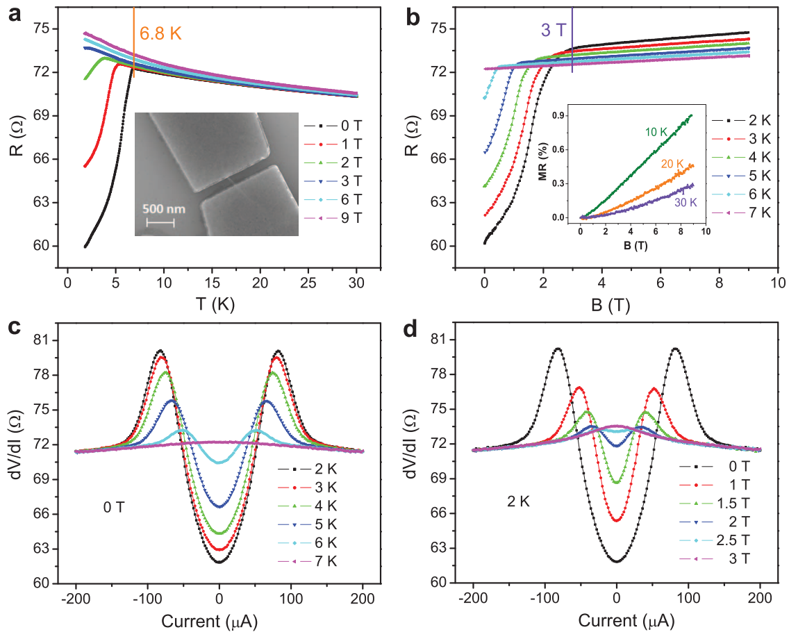
Figure 2 | Electrical transport data of a single DWCNT bundle sample Z-14. (a) Resistance as a function of temperature at a magnetic field B = 0, 1, 2, 3, 6 , and 9 T, (left) from bottom to top, measured with a 1\mu\text{A} DC current. The inset shows its SEM image. (b) Magnetoresistances at temperature T = 2, 3, 4, 5, 6 , and 7 K, (left) from bottom to top. The inset shows magnetoresistances at a higher temperature range T = 10, 20 and 30 K, from top to bottom. (c) Differential resistance at zero magnetic field as a function of current at temperature T = 2, 3, 4, 5, 6 and 7 K, (center) from bottom to top. (d) Differential resistance at 2 K as a function of current at a magnetic field B = 0, 1, 1.5, 2, 2.5 , and 3 T, (center) from bottom to top.
