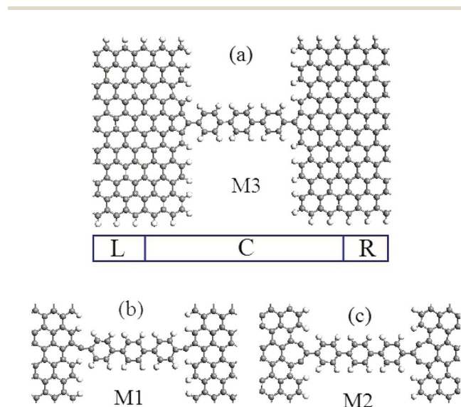
Fig. 1 (a) The geometric structures of model M3, (b) and (c) correspond to the different connection interfaces between the electrodes and the central molecule for models M1 and M2. L (R) and C indicate the left (right) electrodes, and the central scattering region, respectively.
