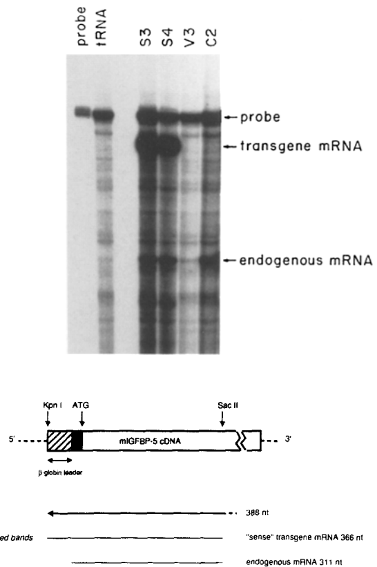
Figure 2. Two independent colonies express IGFBP-5 transgene mRNA. The top panel is an autoradiograph of a ribonuclease protection experiment using 10 μg of total cellular RNA isolated from cells stably transfected with the IGFBP-5 transgene (cell lines S3 and S4) and grown to ~80% confluence in DME containing 20% serum. Total RNA from parental C2 cells (C2), or cells transfected with the empty expression vector (V3), were included as positive controls for the endogenous IGFBP-5 mRNA. Migration of the bands protected by the transgene, the endogenous gene, or the undigested probe are indicated by the arrows on the right. Autoradiographic exposure was for 18 h at -80°C with two intensifying screens. The bottom panel is a schematic representation of the riboprobe derived from the transgene which was used in this experiment to discriminate between mRNAs which contain the β-globin sequence and those which do not.
