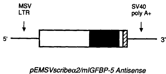
Figure 1. Schematic representation of the pEMSVscribeα2/mIGFBP-5 sense ( top panel ) and antisense ( bottom panel ) expression plasmids were constructed as described in Materials and Methods. The white boxes represent cDNAs corresponding to IGFBP-5 mRNA untranslated sequences. The black boxes indicate the IGFBP-5 coding sequences, while the hatched boxes represent the 55-bp rabbit β-globin 5' untranslated sequence from the pBAT vector. The Moloney sarcoma virus promoter (MSV LTR) and SV40 polyadenylation sequences are marked by arrows.
