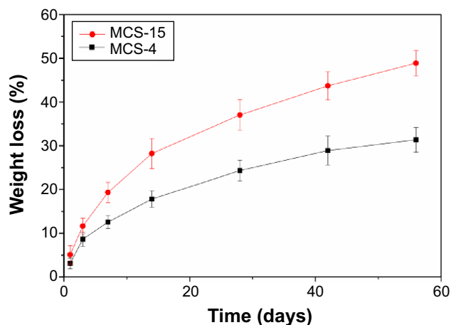
Figure 8 Weight loss of MCS-15 and MCS-4 immersed in Tris-HCl solution with time. Abbreviation: MCS, mesoporous calcium–silicon.
