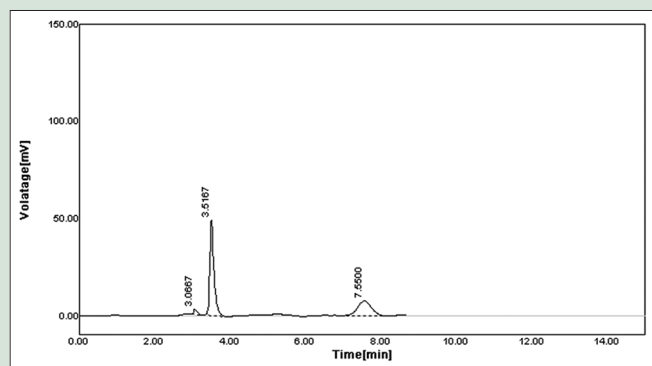
Figure 9: Chromatogram of accuracy 80%
