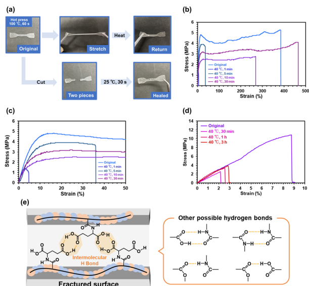
Fig. 5 (a) Photos of original, stretched, and recovered P(nBA-co-AGluOH) sample and preliminary healing test. Stress–strain curves of (b) and (c) P(nBA-co-AGluOH) after healing in (b) 0–500% strain and (c) 0–50% strain, and (d) P(nBA-co-AThrOH) after healing and (e) schematics of healing process of P(nBA-co-AGluOH) .
