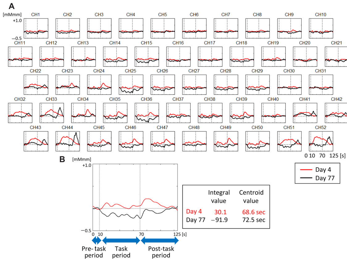
Figure 2 Waveforms of oxygenated hemoglobin. Notes: (A) Waveforms of oxygenated hemoglobin during the cognitive activation of the word fluency task. (B) Grand average waveforms of oxygenated hemoglobin in the frontal region (CH 25, 26, 27, 28, 36, 37, 38, 46, 47, 48, and 49).
