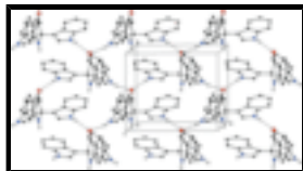
Fig. 2. Part of the crystal structure of (I) showing the hydrogen bonded layers parallel to the ab plane. Intermolecular hydrogen bonds are shown as dashed lines and H atoms not involved in H-bonding have been omitted.
