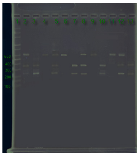
Fig. 1. Representative gel of XRCC1 Arg399Gln polymorphism, showing MspI digested amplicons. The Arg allele is represented by 374 and 241-bp fragments, while the Gln allele is represented by a 615-bp band. Lane 1, 100-bp ladder; lanes 4, 6, 9, and 11, homozygous (Gln/Gln) genotype (615 bp); lanes 3, 7, 10, and 13, homozygous (Arg/Arg) genotype (374 and 241 bp); lanes 2, 5, 8, and 12, heterozygous (Gln/Arg) genotype (615, 374 and 241 bp).
