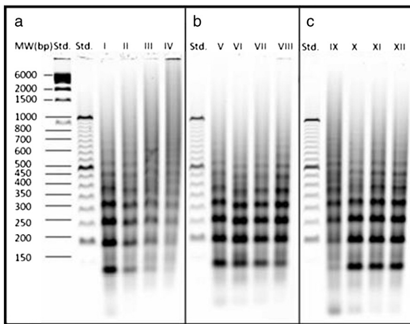
Fig. 3. Electrophoretic analysis of the DNA concatemers formed in the presence of added 200 mM NaCl, under the following conditions. (a) Oligo concentrations: 2.5, 5, 10, and 20 \mu\text{M} (lanes I–IV). (b) Incubation temperatures: 4, 20, 37 and 60 ^{\circ}\text{C} (lanes V–VIII). (c) Incubation times: 2, 24, 48 and 72 h (lanes IX–XII). Electrophoresis in 2.5% agarose gels at 4 V/cm.
